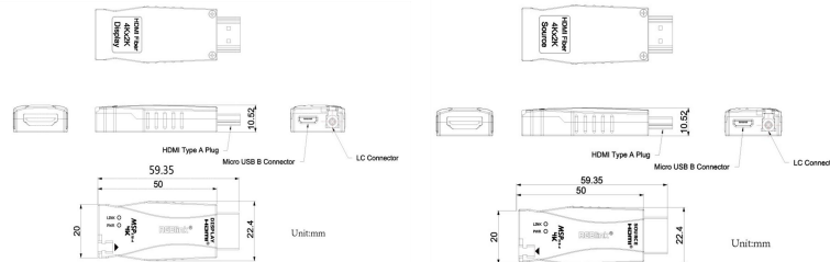
MSP 318-4 Transmitter
